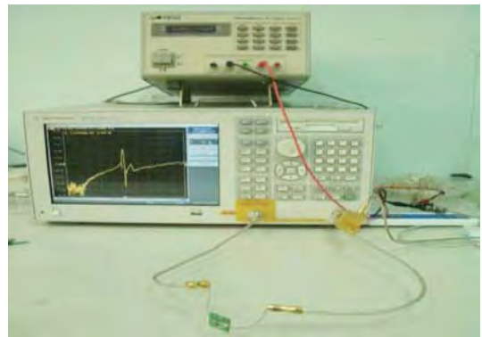
Fig.4 Network Analyzer
